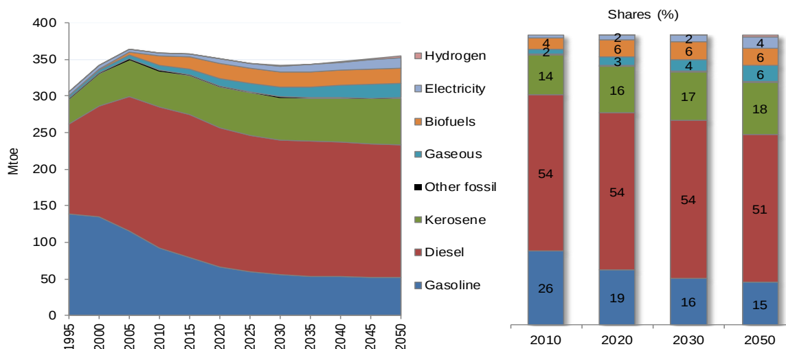
Figure 16: Final energy demand in transport by fuel type
