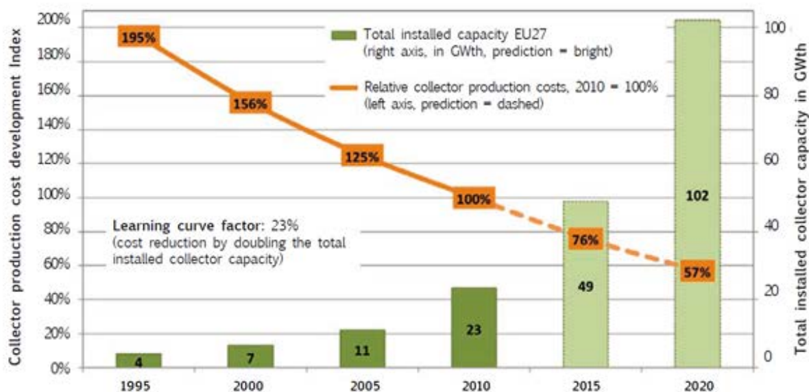
Figure 8: Costs for high-efficient flat plate solar collector panel (of about 2.2 to 2.5 m 2 gross collector area) manufactured in Europe 216
